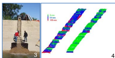
Figure 2,3 & 4: Simulation test site along with terrestrial LIDAR measured erosion
